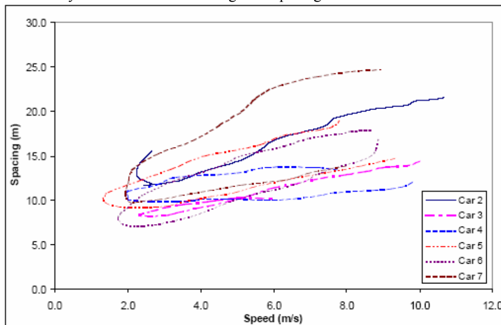
Figure 1 Spacing of individual vehicles in platoon
