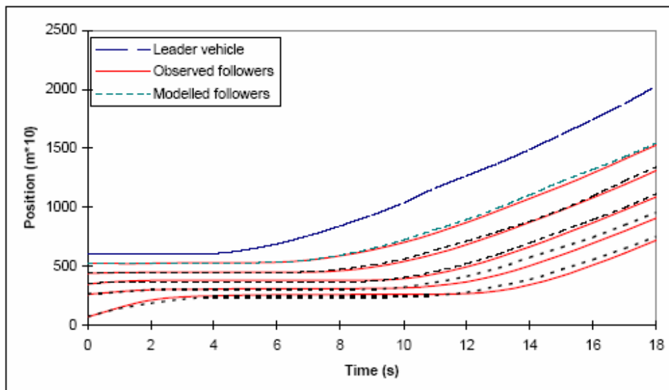
Figure 2 Comparison of measured and modelled trajectories (platoon 6)
