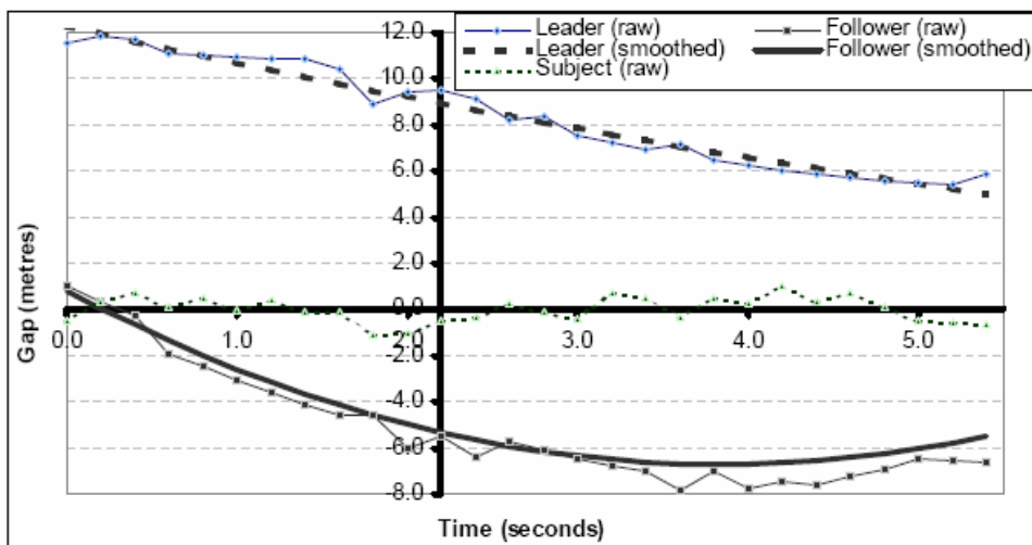
Figure 6 Cooperative lane change (observed)
