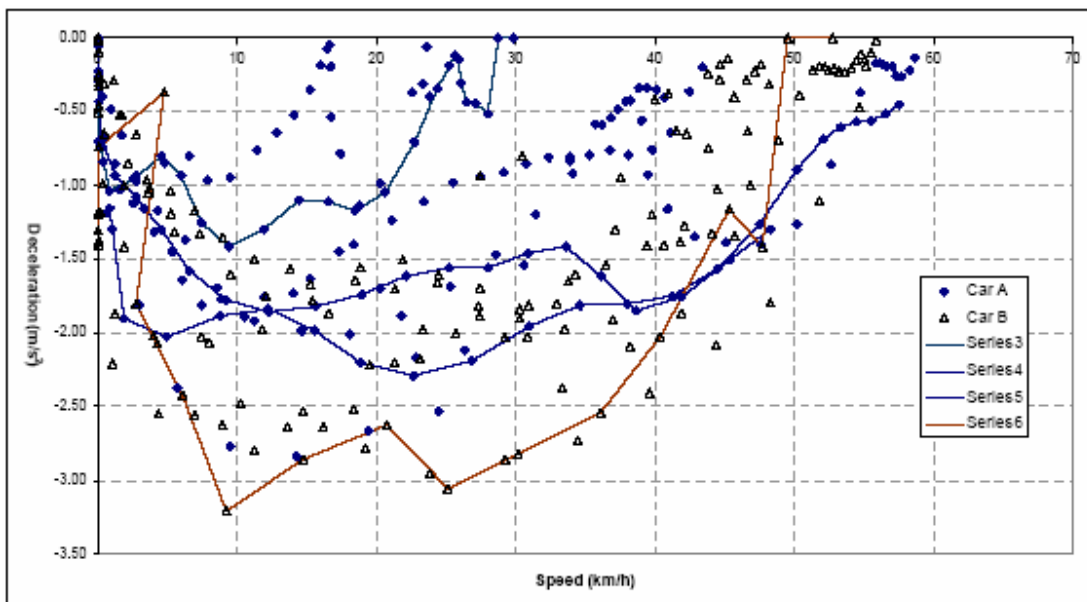
Figure 10 Deceleration vs. Speed
