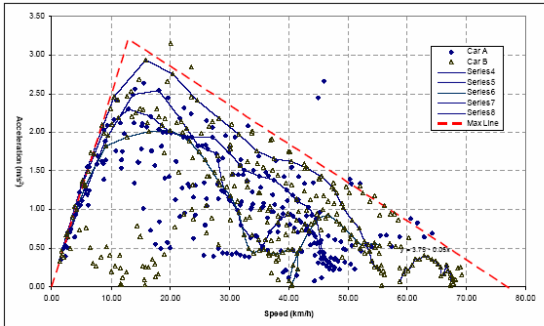
Figure 9 Acceleration vs. Speed
