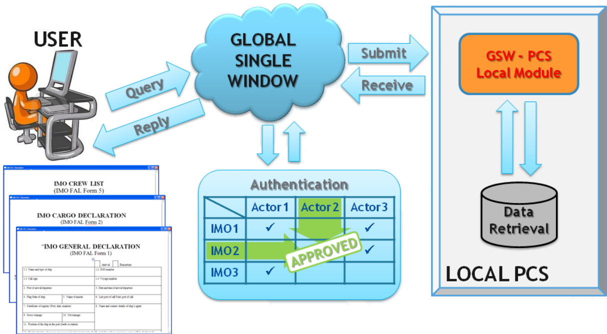
Figure 3 - Communication schema between Global Single Window and local PCS
