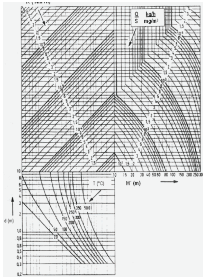
Figure 1 - Estimation of chimney heights in Bogota according to emission rates and operating temperatures.
