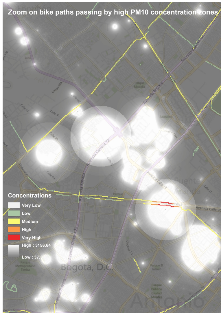
Figure 12 – Map of high PM 10 concentrations along bicycle paths
