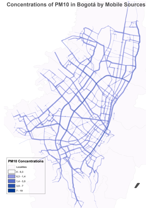
Figure 8 – Map: PM 10 Concentrations in Bogotá due to mobile sources
