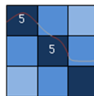
Identification (in red) of bicycle paths pieces passing by high PM 10 concentrations.
