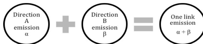
Figure 6 - Sum of the two directions to form one source, one link
