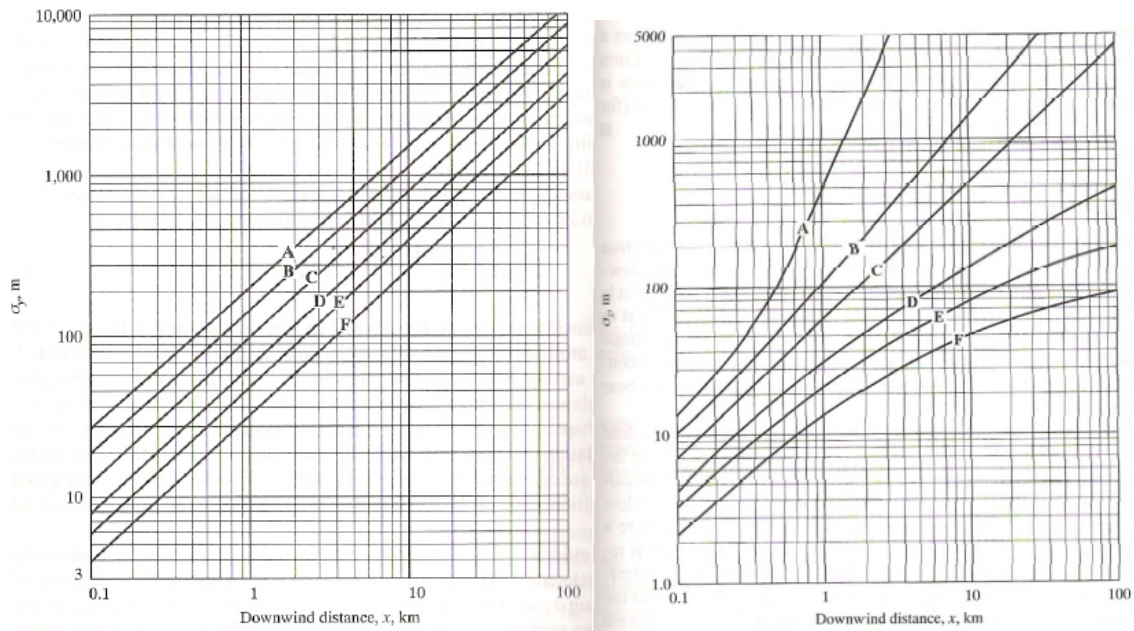
Figure 2 - Charts for the definition of vertical and horizontal dispersion coefficients (From Wang et al. 2004)
