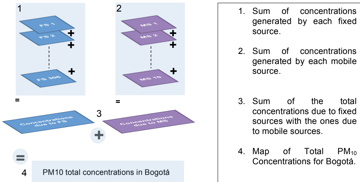
Figure 5 - Modelling part 1 scheme
