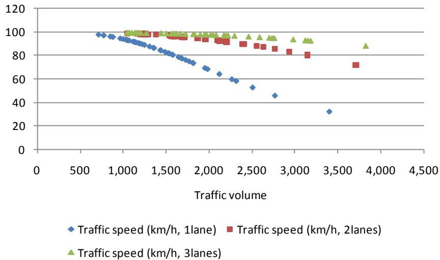
Figure 11 – Relationship between traffic volume and expressway traffic speed
