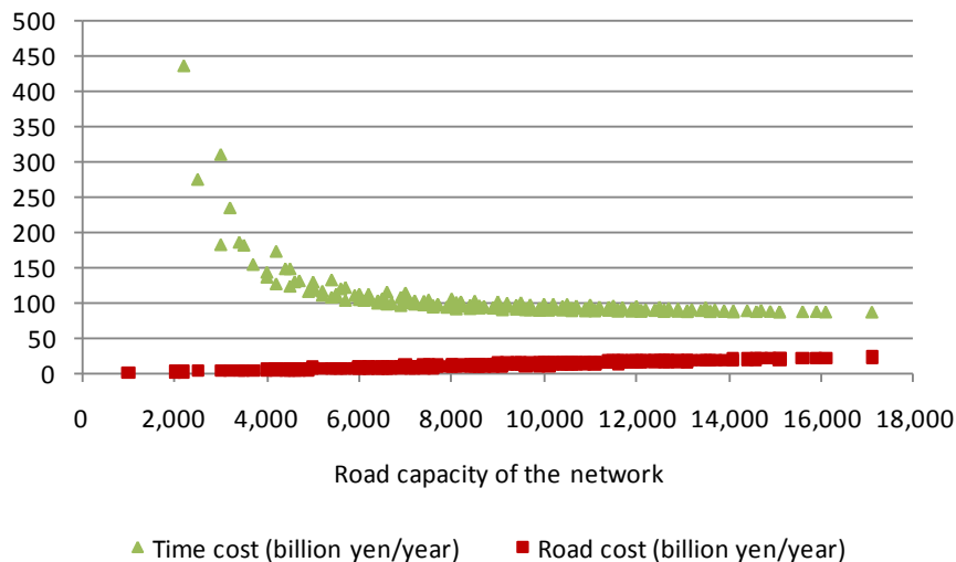
Figure 6 – Relationship between road capacity, time cost of road users and road cost (Cross traffic volume is 4,500 vehicles/hour)
