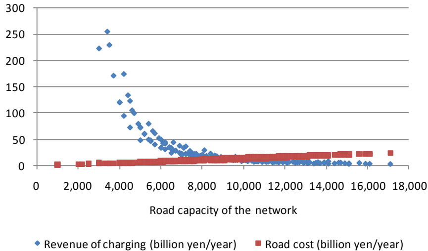
Figure 5 – Relationship between road capacity, revenue of charging and road cost (Cross traffic volume is 4,500 vehicles/hour)
