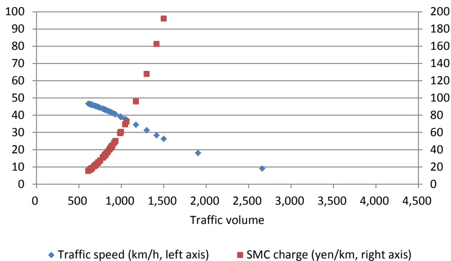
Figure 9 – Relationship between traffic volume and traffic speed or SMC charge in one lane of arterial highway
