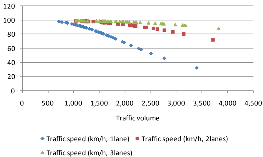
Figure 17 – Relationship between traffic volume and sub-arterial highway traffic speed
