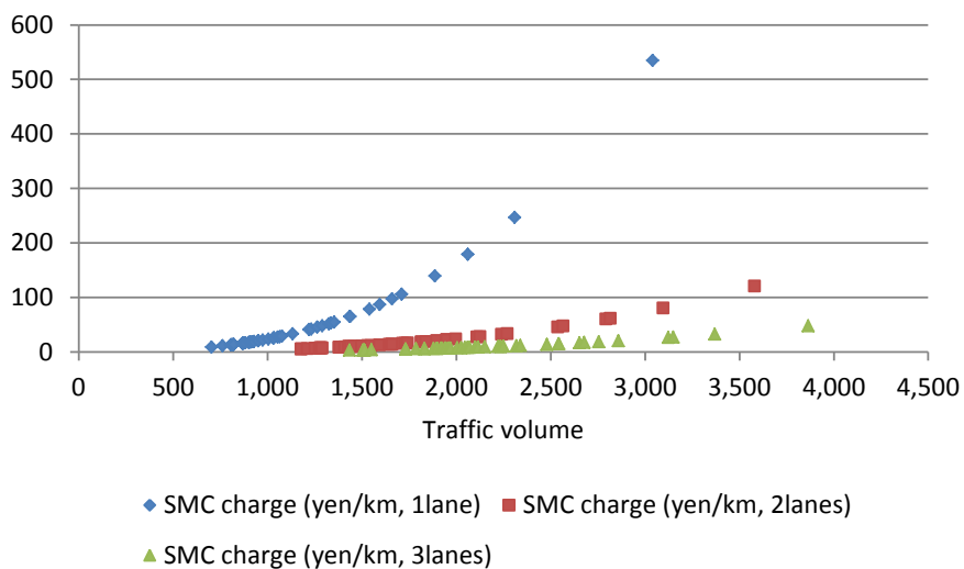
Figure 14 – Relationship between traffic volume and SMC charge in main arterial highway
