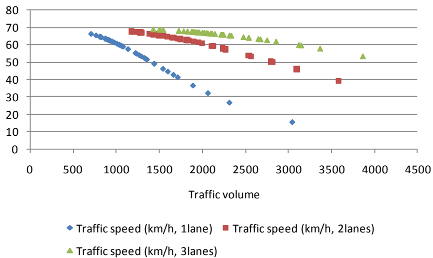
Figure 13 – Relationship between traffic volume and main arterial highway traffic speed
