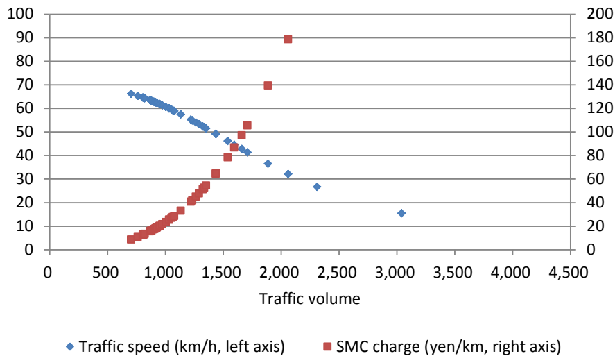
Figure 8 – Relationship between traffic volume and traffic speed or SMC charge in one lane of main arterial highway
