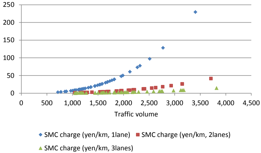
Figure 12 – Relationship between traffic volume and SMC charge in expressway
