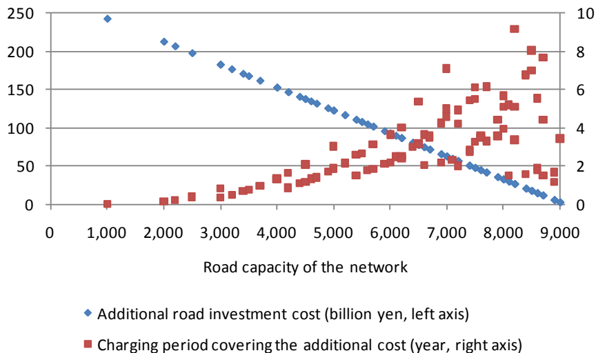
Figure 19 – Relationship between additional road investment cost and charging period covering the additional cost
