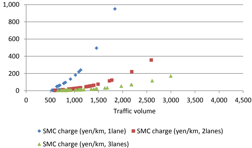
Figure 18 – Relationship between traffic volume and SMC charge in sub-arterial highway
