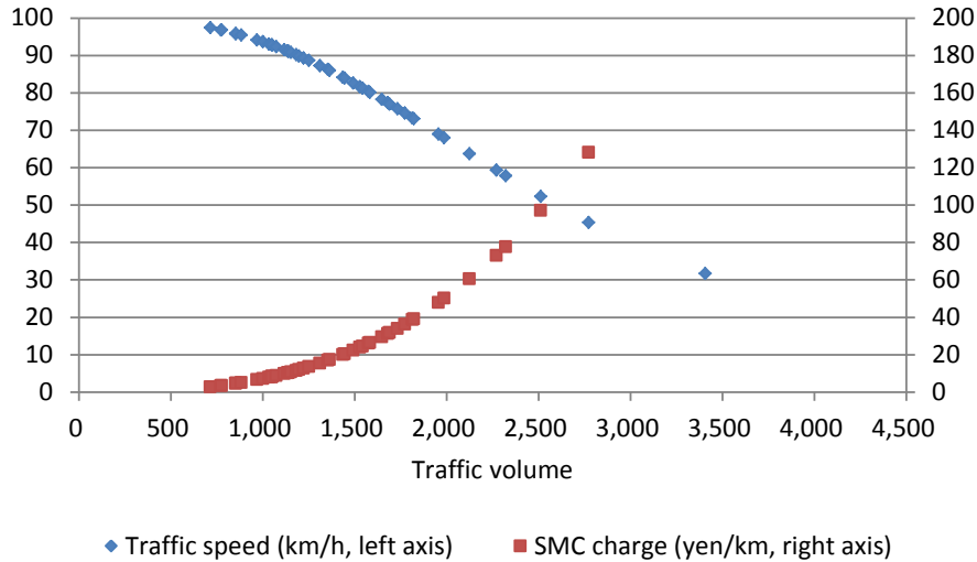
Figure 7 – Relationship between traffic volume and traffic speed or SMC charge in one lane of expressway
