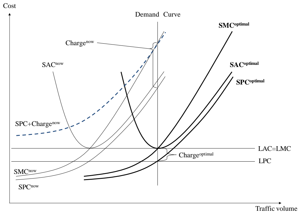
Figure 4 – SMC charging in fixed demand
