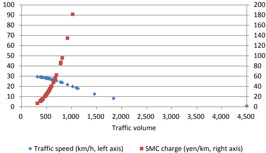
Figure 10 – Relationship between traffic volume and traffic speed or SMC charge in one lane of sub arterial highway
