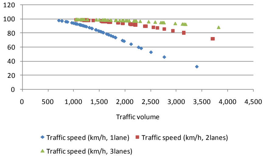
Figure 15 – Relationship between traffic volume and arterial highway traffic speed
