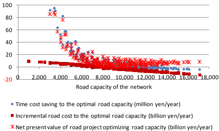
Figure 20 – Relationship between road capacity and net present value of road project optimizing road capacity
