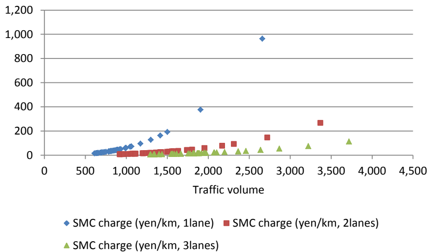
Figure 16 – Relationship between traffic volume and SMC charge in arterial highway
