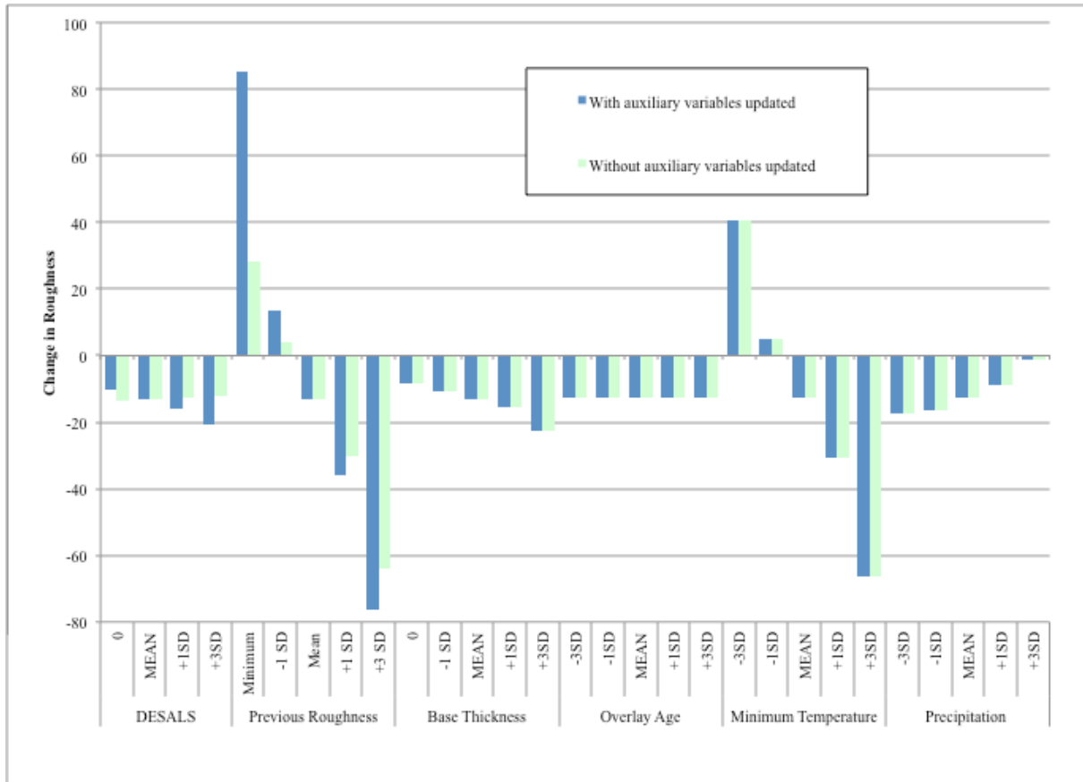
Figure 2 – Effect of different parameters on predicted change in roughness
