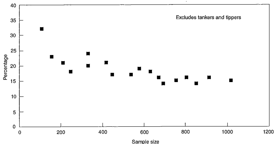
Figure 6 Calculated percentage of empty running based on varying sample sizes
