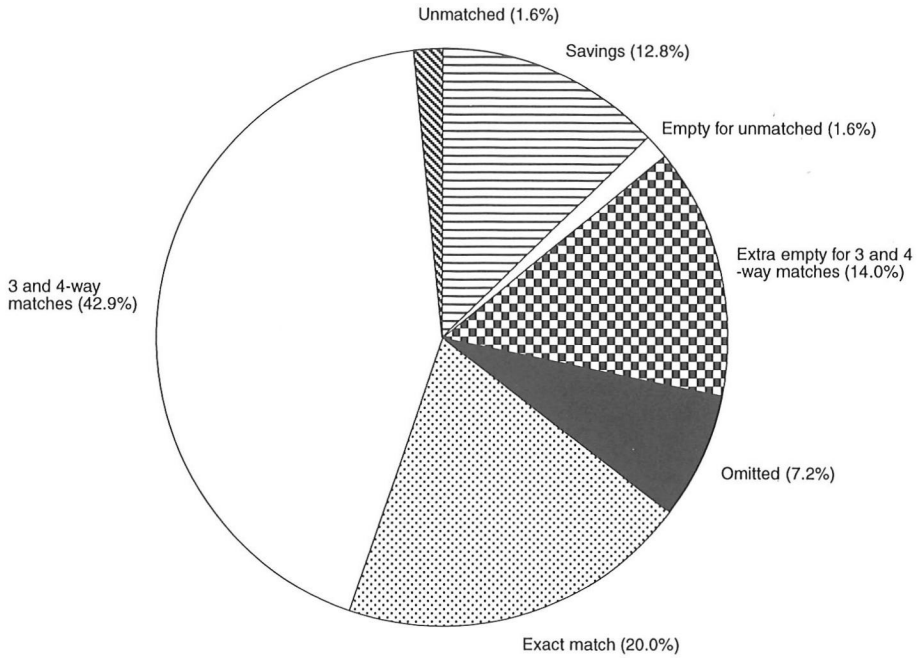
Figure 4 Potential savings in empty running—loaded matching analysis
