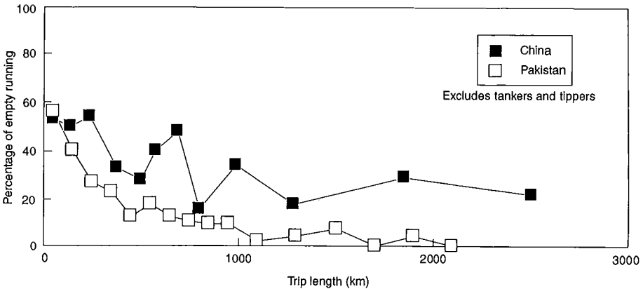
Figure 2 Distribution of empty running
